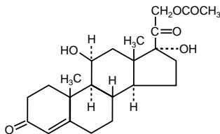
hydrocortisone acetate (pregn-4-ene-3,20-dione, 21-(acetyloxy)-11,17-dihydroxy-, (11β)-) C 23 H 32 O 6 ; mol. wt. 404.50
